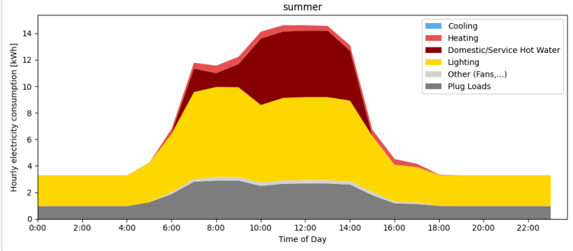
Average daily consumption profile for winter and summer, showing the contribution of cooling, lighting, domestic hot water, plug loads, and auxiliary systems throughout an average winter and summer day.
